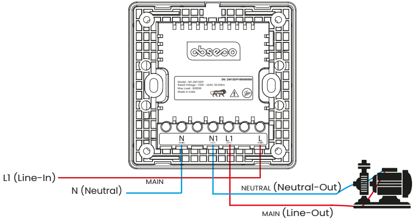
Figure 1: Wiring Diagram
